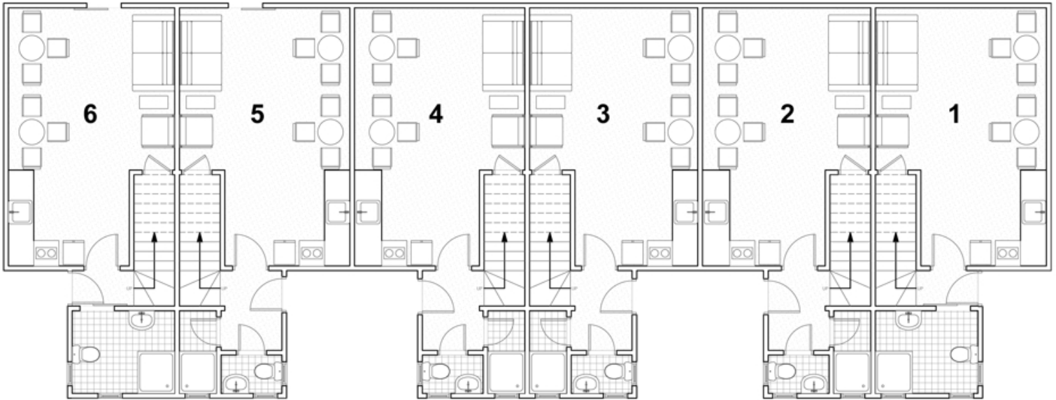
LOWER FLOOR PLAN.
