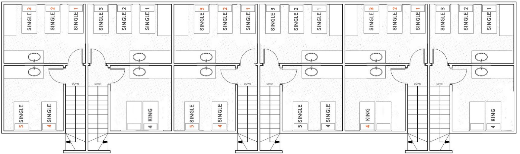
UPPER FLOOR PLAN.
